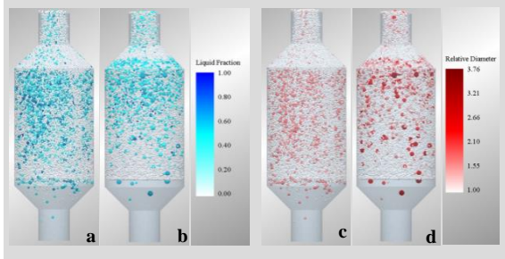
Fluidized bed granulation
