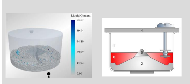
High-shear granulation
