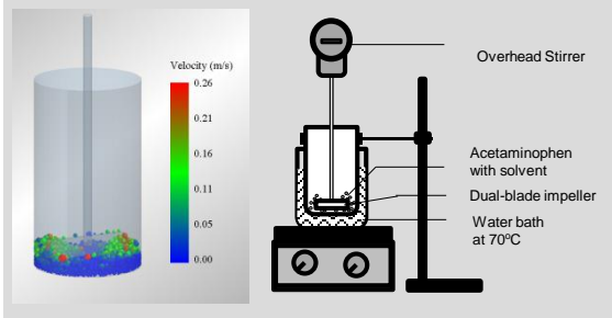
Agitated Filter Dryer
